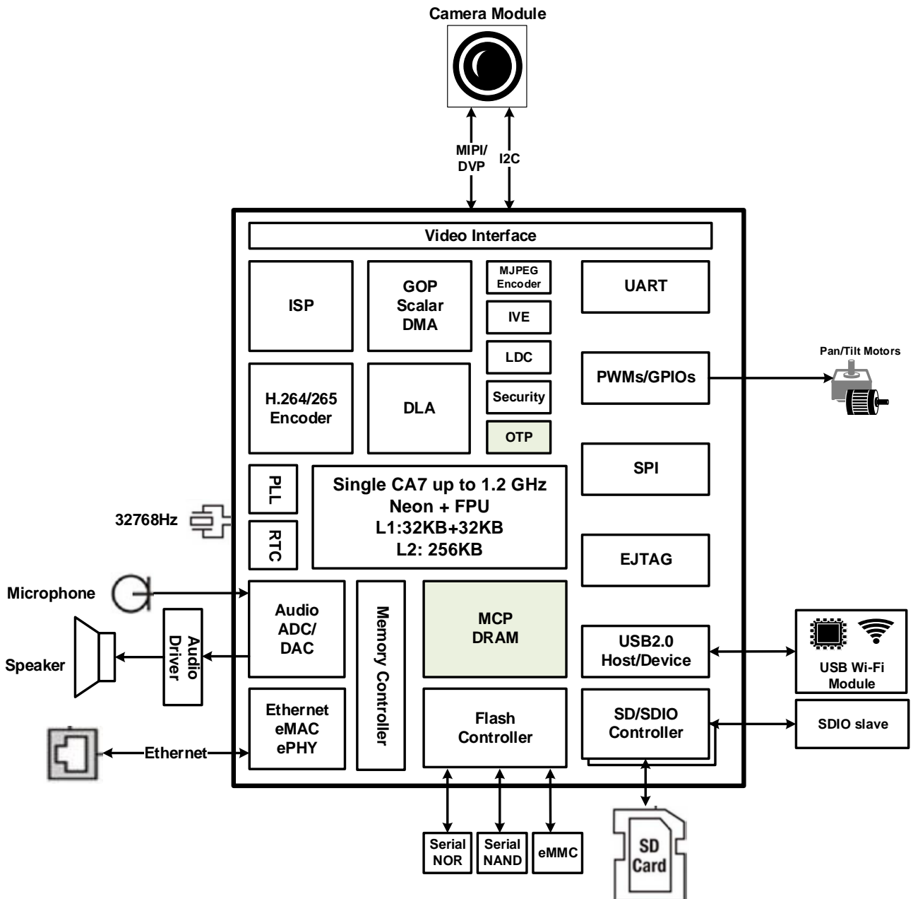
Figure 0-1: SSC30KD/SSC30KQ Block Diagram
